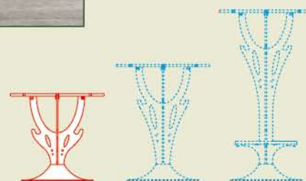
Example of combination of table model TI 110.80 and additional square top model AI 400.80 (optional).
